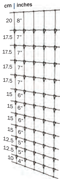
13/190/15 Intensive boundary/Emu
