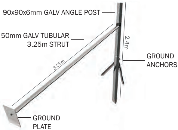
Drive-In End Assembly
