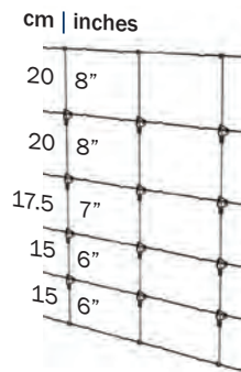
6/90/30 Cattle
