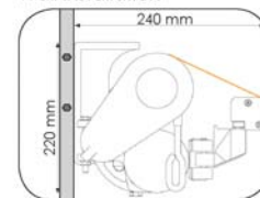
Wall installation
