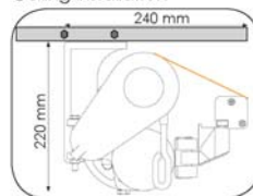
Ceiling installation
