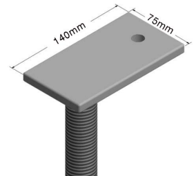
End Of Bearer 10mm Thick 14mm Bolt Hole Code: E
