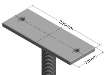
Straight 10mm Thick 14mm Bolt Holes Code: S
