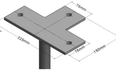
Tee 10mm Thick 14mm Bolt Holes Code: T
