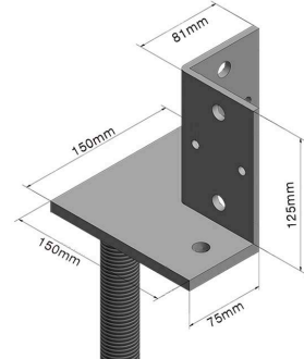
Vertical Large Corner 10mm Thick 8mm & 14mm Bolt Holes Code: VLC
